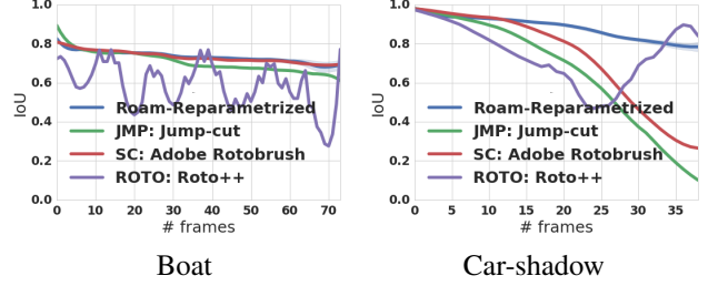
Figure 7: Evolution of IoU for different sequences of the DAVIS dataset. For our method, the blue shadow indicates influence of varying the label space size for each node (set of possible moves in dynamic programming inference).
