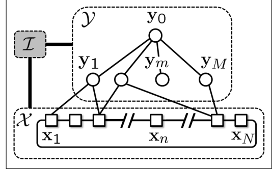
Figure 2: Graphical model of ROAM . In joint model defined by energy E(\mathcal{X}, \mathcal{Y}; \mathcal{I}) in (1), contour node variables (white squares) form a closed 1-st order chain conditioned on image data (grey box) and landmark variables (white circles), the latter variables forming a shallow tree conditioned on all others.
