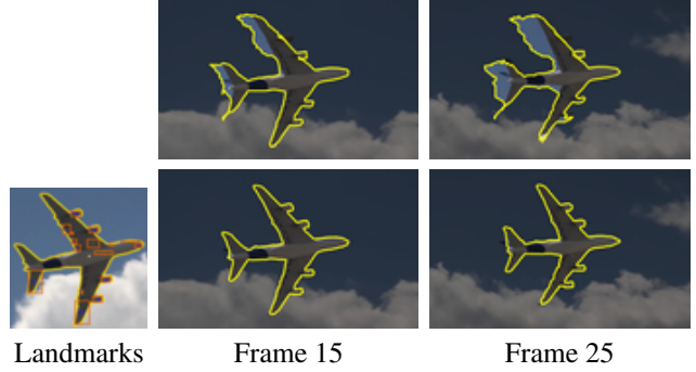
Figure 8: Benefit of landmarks-based modeling. Automatically detected landmarks (orange bounding boxes) are accurately tracked on the plane sequence. This further improves the control of the boundary (bottom), as compared to ROAM without landmarks (top).
